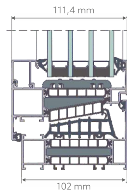
CROSS SECTION OF WINDOW TM 102HI
